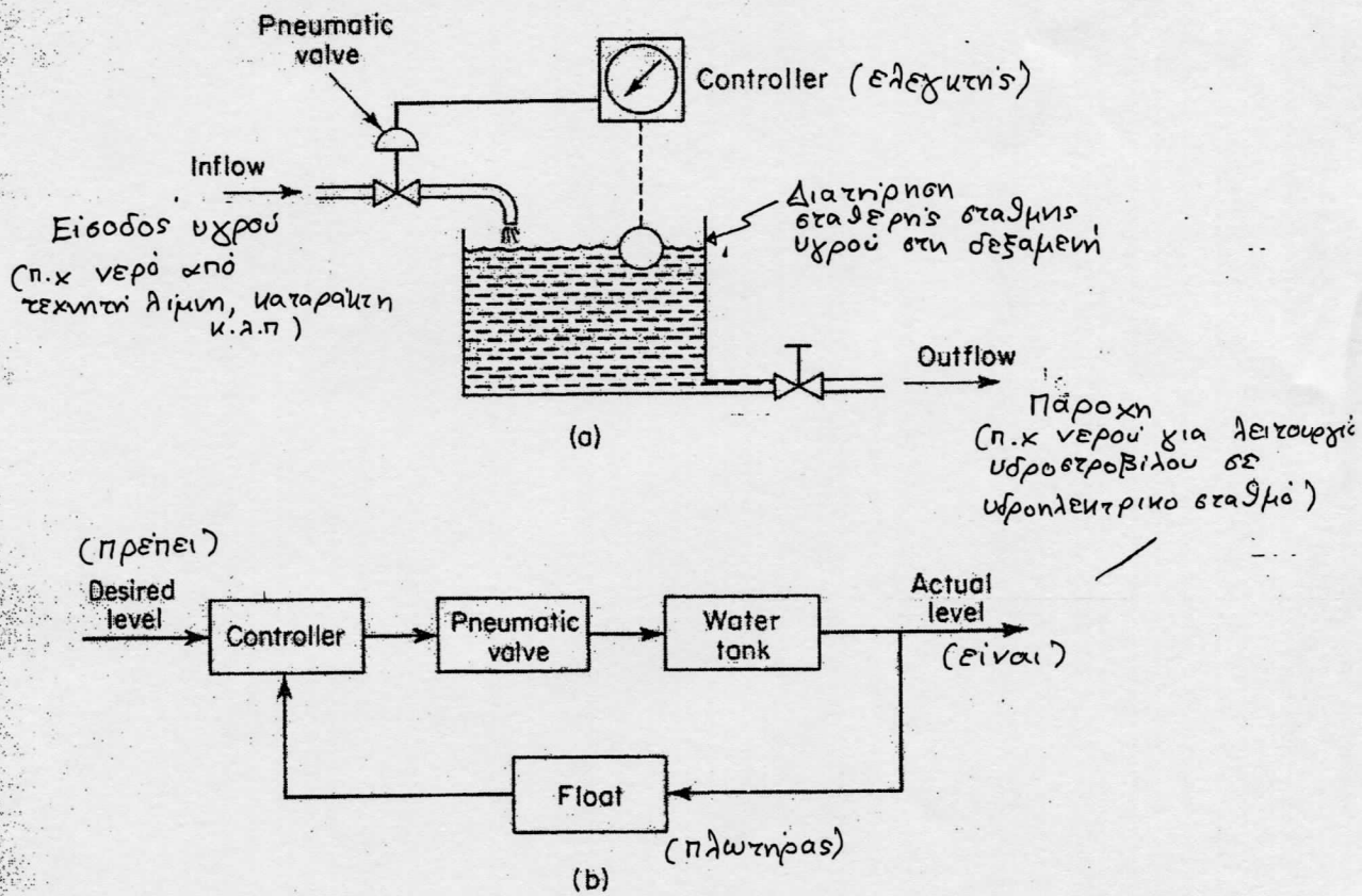
Fig. 1-10. (a) Liquid-level control system; (b) block diagram.
